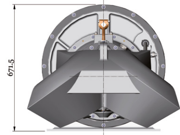
OUTBOARD VIEW OF ULTRAJET UNIT
