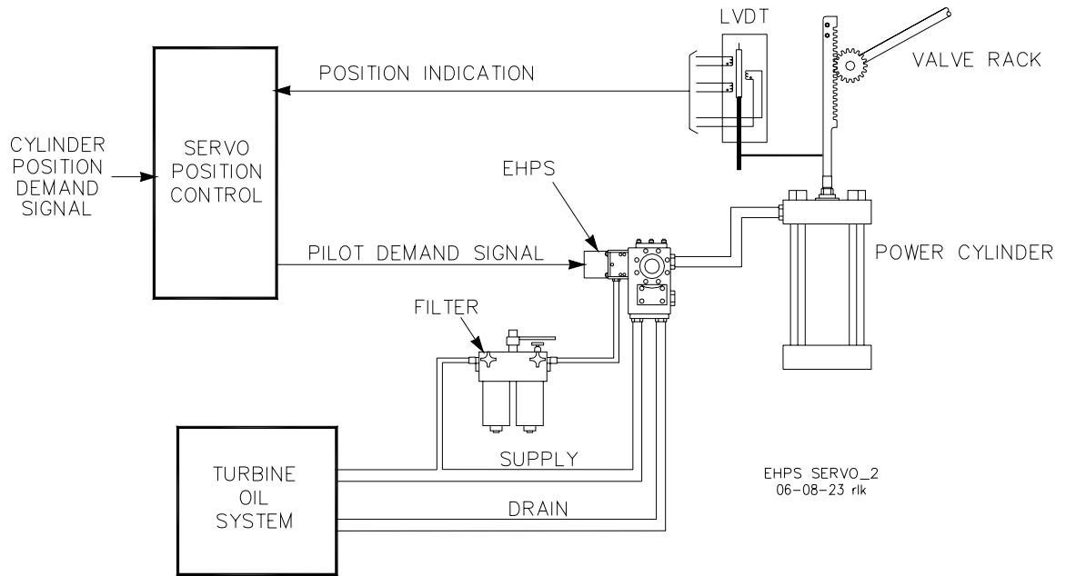
Figure 3. Typical EHPS Application—Single Acting Actuator
