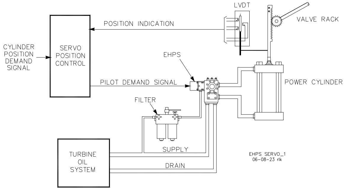
Figure 2. Typical EHPS Application—Double Acting Actuator
